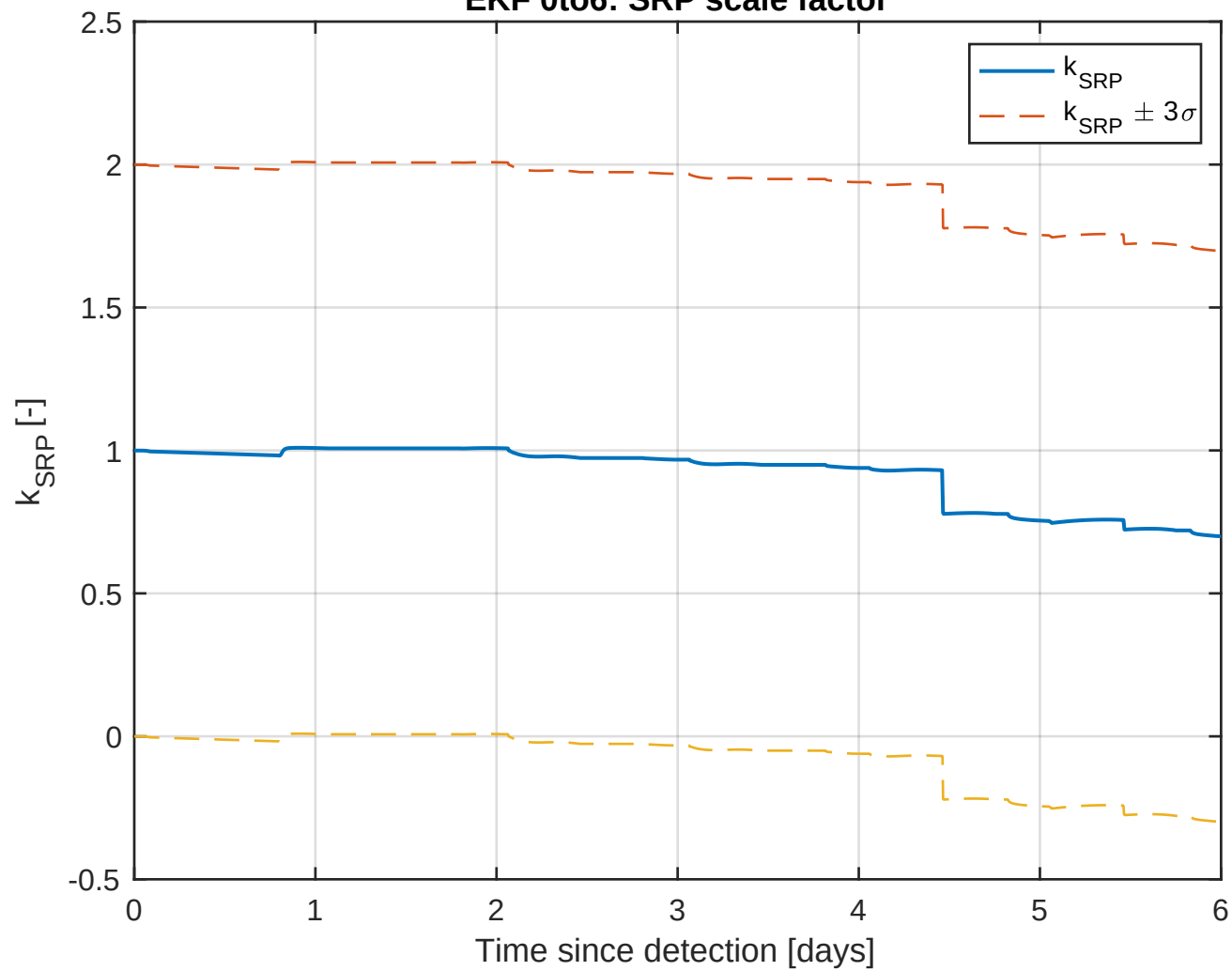
EKF 0to6: SRP scale factor
